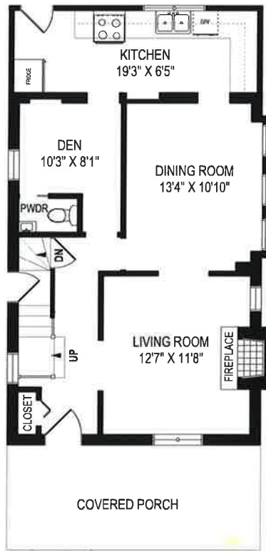
MAIN FLOOR PLAN 709 SQUARE FEET CEILING HEIGHT 8'10"
